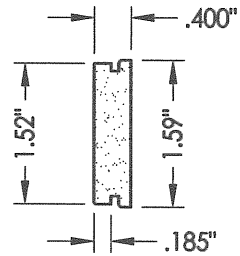
43 LATCH & HINGE STILE Cellular PVC
