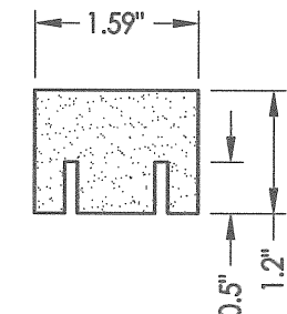
45 BOTTOM RAIL Cellular PVC
